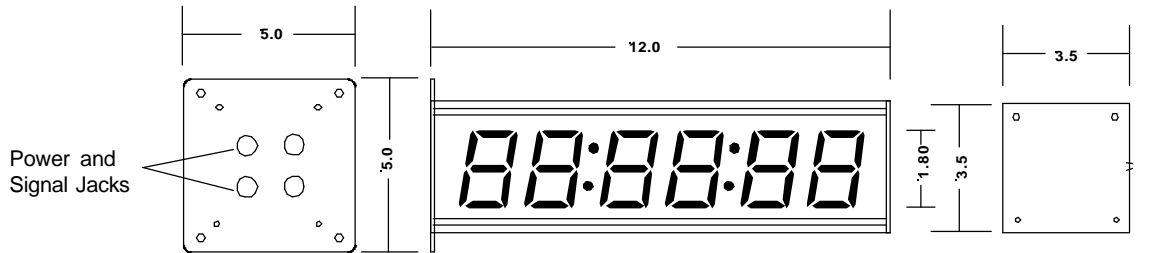
Optional Wall Mount Plate for Single or Double-Sided models
